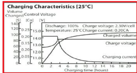
Charging Characteristics
