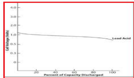
Discharging Characteristics
